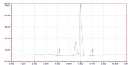
Figure 9: UV Light degradation chromatogram.
