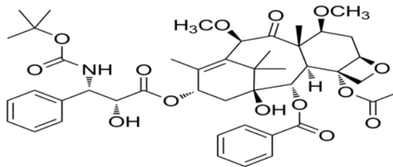
Figure 1: Structure of Docetaxel.
