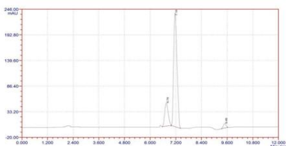
Figure 7: Peroxide degradation chromatogram.
