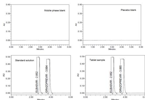
Figure 2: Chromatograms of selectivity studies.
